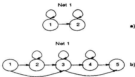
Fig. 5. State transition diagrams of the HCNN model.
