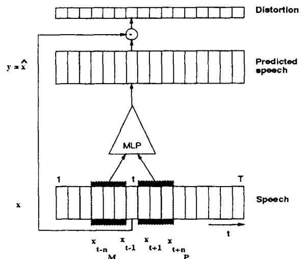
Fig. 1. Predictive connectionist modeling principle for ASR.
