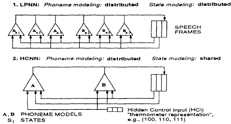
Fig. 2. LPNN and HCNN modeling principles.
