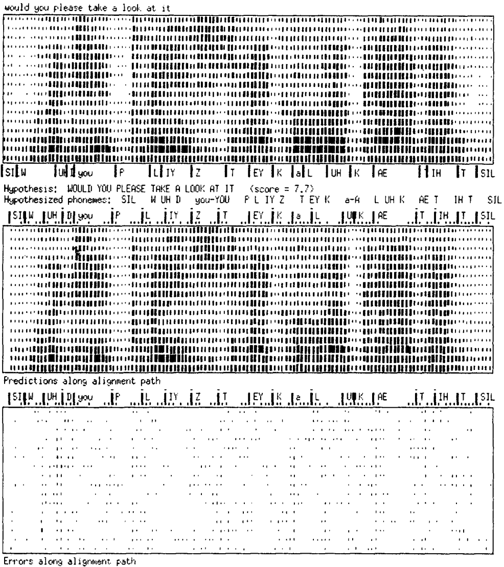
Fig. 6. Typical example of the HCNN-CDF continuous speech recognition. Upper trace: Actual sentence. x-axis: time (frame sampling rate is 10 ms); y-axis: frequency (normalized melscale filterbank coefficients). Middle trace: Predictions and segmentation generated by the HCNN system. Major hash marks: phoneme and function word boundaries; Minor hash marks: HCNN-input "thermometer" input change; Bars above major segmentation marks specify the alternate model index. Lower trace: Prediction errors made along the alignment path.
