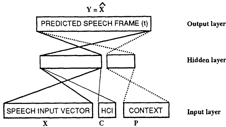
Fig. 4. Context-dependent HCNN model.
