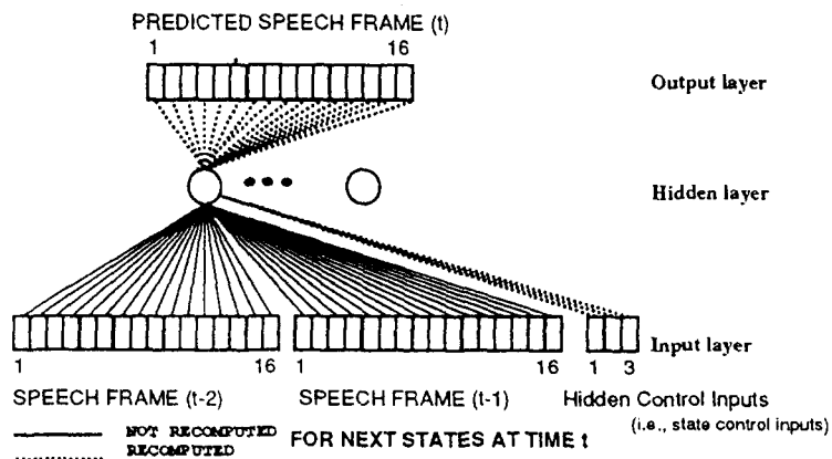
Fig. 3. Reduction of computational load by the HCNN modeling principle.
