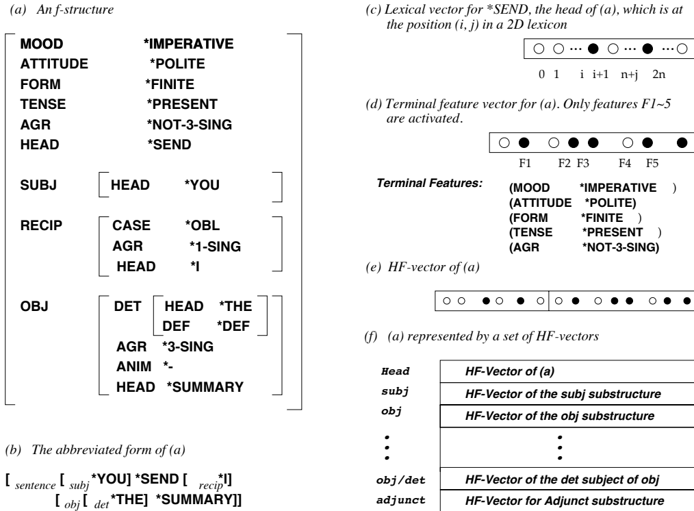
Figure 1: F-structure Representation. (a) an f-structure. (b) abbreviation. (c). lexical vector. (d). terminal feature vector. (e) HF-vector. (f) f-structure represented by HF-vectors.
