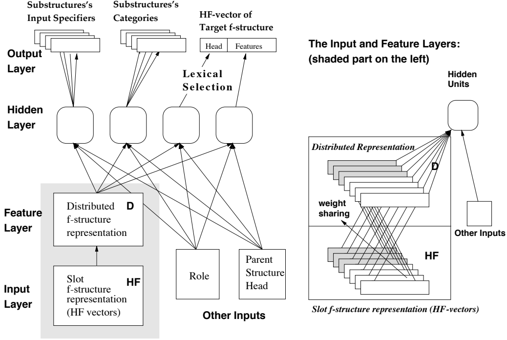
Figure 2: Phrasal Network Structure. (a): the architecture of a phrasal network. (b): details of the lowest two layers. The unshaded slots represent the input f-structure. The shaded ones represent the context f-structure.
