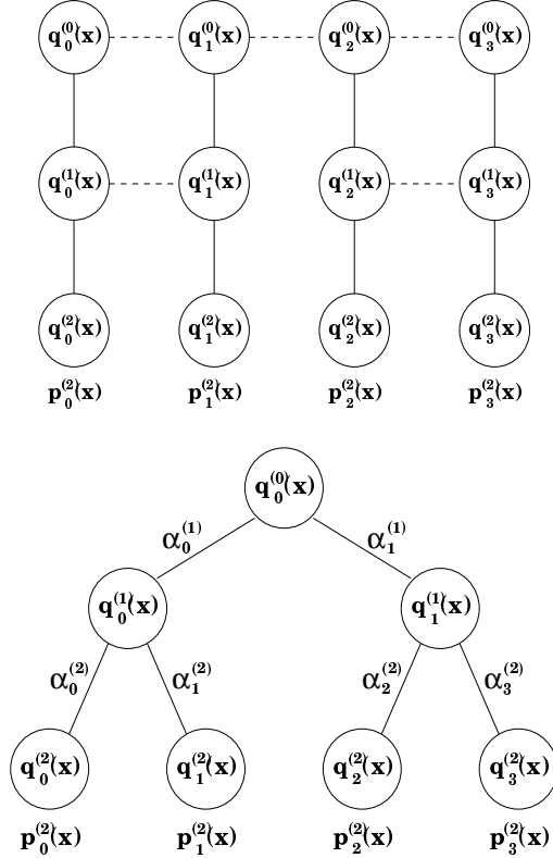
Figure 1. Hierarchically Tied Mixture Densities ( d = 2, b = 2 )
