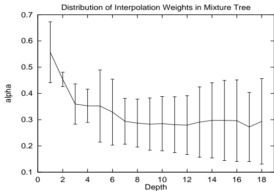
Figure 2. Distribution of Interpolation Weights in Mixture Tree
