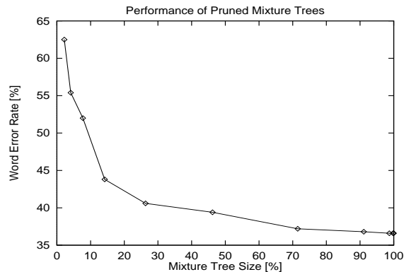
Figure 3. Word Error Rate vs. Tree Size
