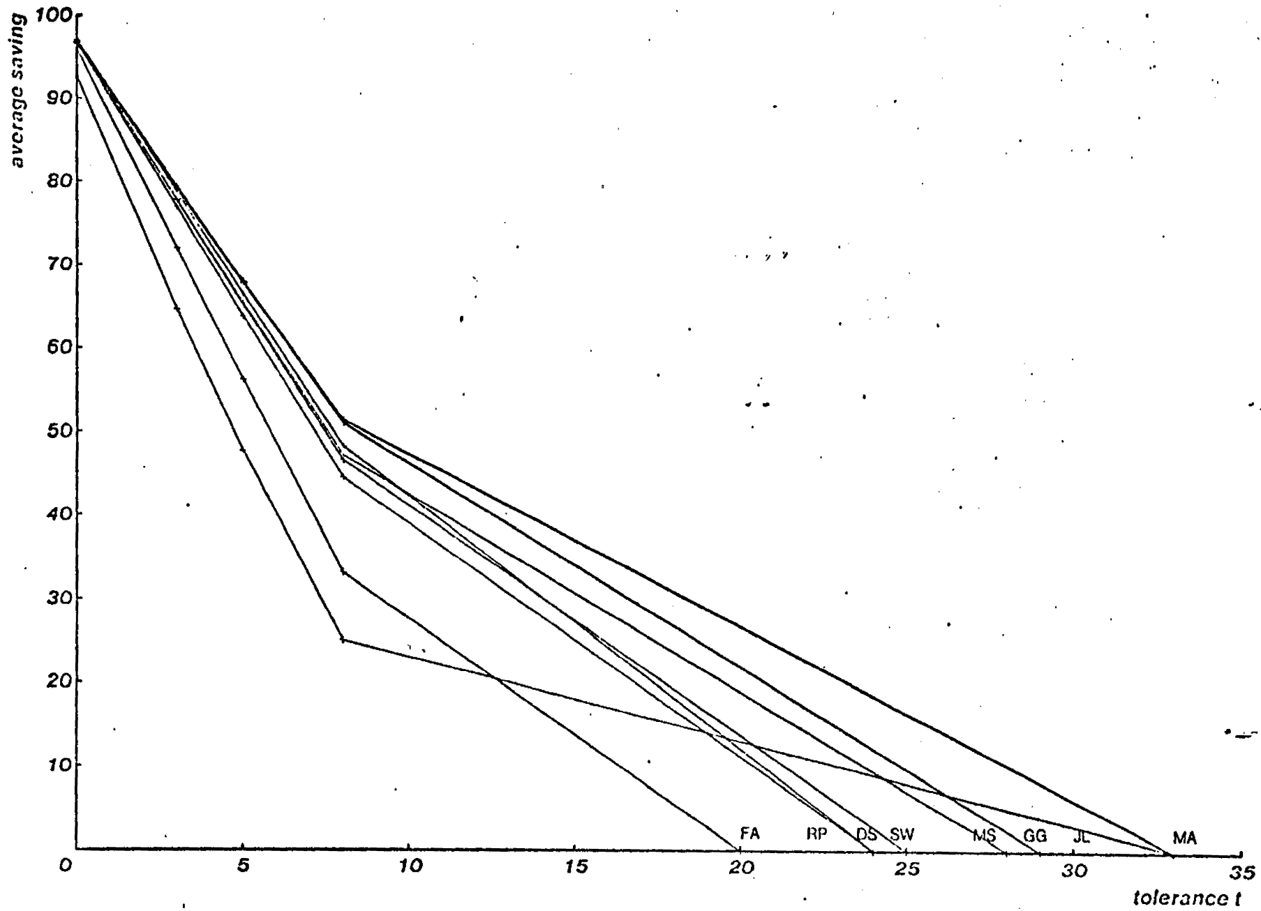
Fig 13 Computational Saving (Confusable vocabulary v2)
