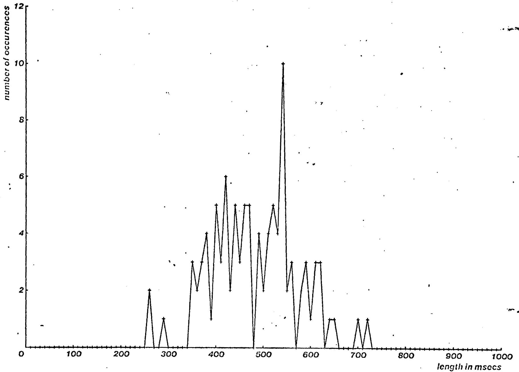
Fig.14 Histogram of digit utterance lengths (speaker FA)
