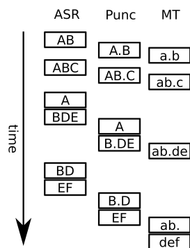
Figure 1: Update Protocol
